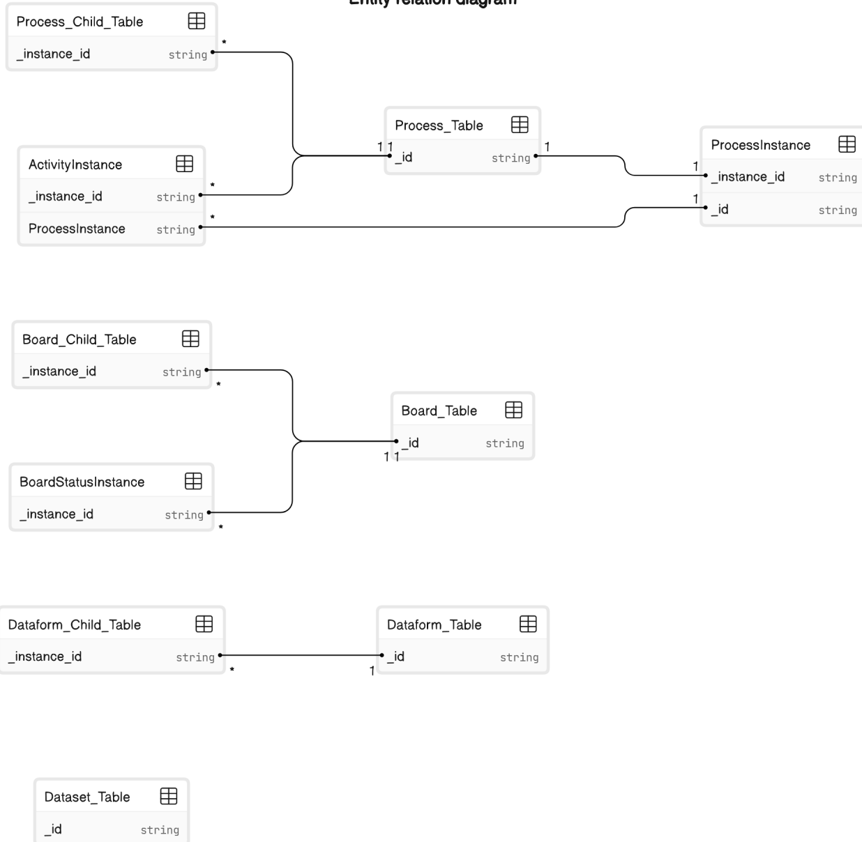
Entity relation diagram
